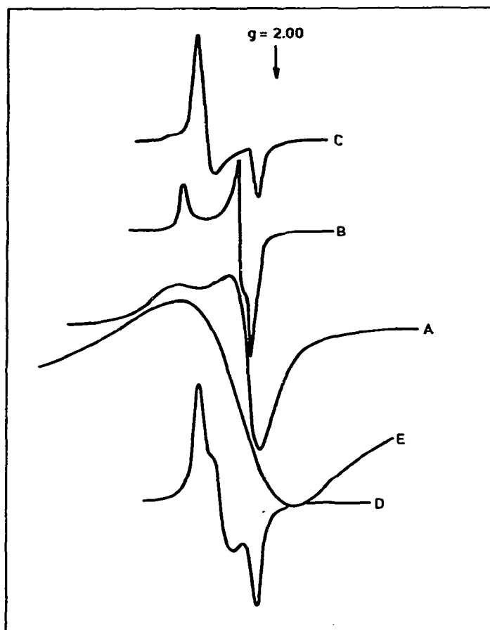
Fig. 7. Typical examples of ESR spectra for cyanato-copper(II) complexes.
