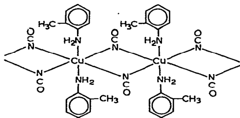
Fig. 6. Assumed structure of \text{Cu}(\text{NCO})_2(\text{o-tol})_2 .
