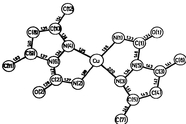
Fig. 12. Structural unit of \alpha\text{-Cu}(\text{3,5-dimethyl-1-carbamylpyrazolate})_2 . Bond lengths in Å. After ref. 109.
