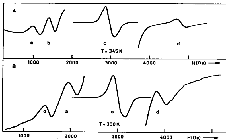
Fig. 10. X-band ESR spectrum of [\text{Cu}_2(\text{tren})_2(\text{NCO})_2](\text{Bph}_4)_2 , form I(A) and form II(B). (a) triplet \leftarrow singlet transition; (b) \Delta M_S = 2 transition; (c) \Delta M_S = 1 transition; (d) triplet \leftarrow singlet transition.
